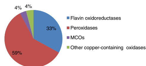
Fig. 4 Relative abundance of the different types of oxidoreductases found in the secretomes of Leptosphaerulina sp. Flavin oxidoreductases (GMC oxidases, NADH oxidases and others), peroxidases (POD, DyPs, catalases), MCOs and other copper-containing oxidases from the nLC-MS analysis and search against Uniprot database (restricted to Ascomycota) are depicted. a. dye-supplemented culture. b. Laccase-induced culture. The total number of oxidoreductase matches is shown in parenthesis (see Additional file 1: Tables S1 and S2 for detailed information)
