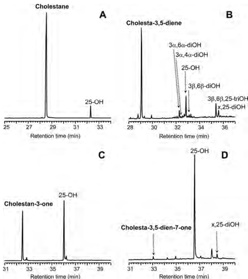
FIG 7 GC-MS analysis of the rCciUPO reaction (at 60 min) with cholestane (A), cholesta-3,5-diene (B), cholestan-3-one (C), and cholesta-3,5-dien-7-one (D) (depicted in Fig. 1) showing the remaining substrates and the mono-, di-, and trihydroxylated derivatives included in Table 4 (x denotes the unknown position of hydroxylation in the ring).
