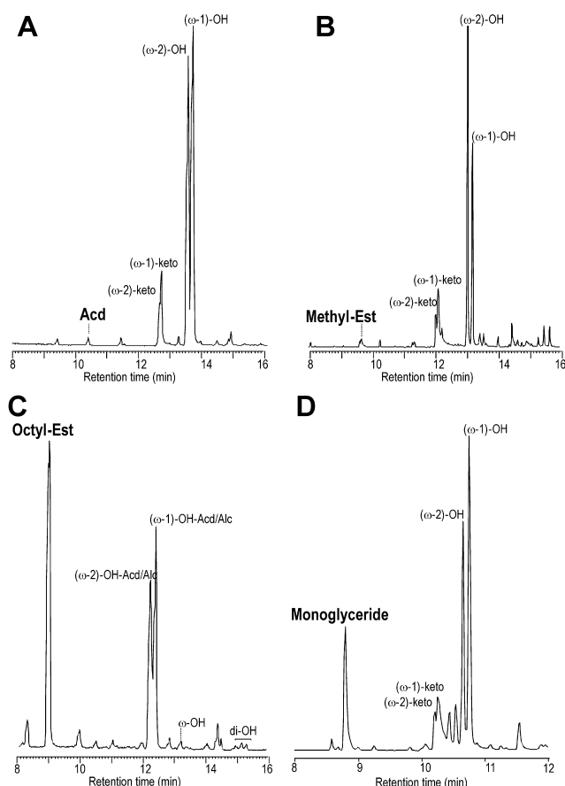
Figure 1. GC-MS analysis of the recombinant C. cinerea peroxxygenase reactions (at 30 min) with myristic acid ( A ), methyl myristate ( B ), octyl octanoate ( C ), and glyceryl myristate ( D ) showing the remaining substrates (Acid, acid; Methyl-Est, acid methyl ester; Octyl-Est, acid octyl ester; Monoglyceride, acid monoglycerol ester) and the \omega -1 and \omega -2 monohydroxy and keto derivatives (Acid/Alc, acid/alcohol).
