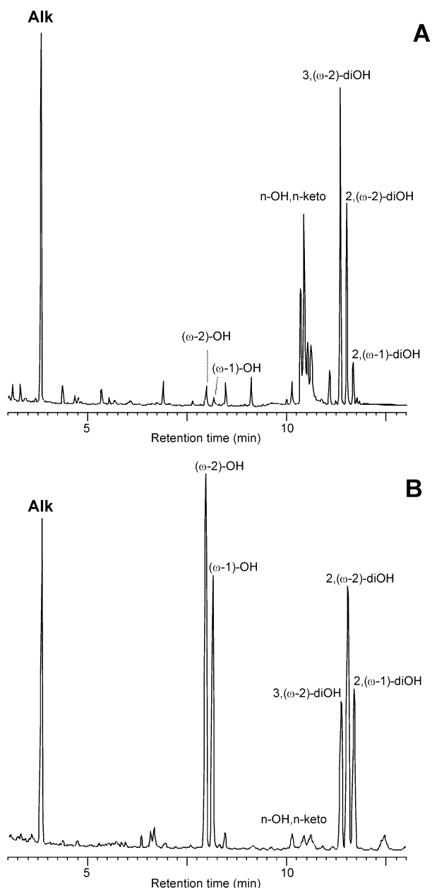
Figure 6. GC-MS analysis of the recombinant C. cinerea peroxxygenase reactions with tetradecane at 120 min in the presence of 20% (A) and 40% (B) acetone, showing the remaining alkane (Alk), and the \omega -1 to \omega -2 monohydroxy, hydroxy-keto, and dihydroxy derivatives formed.
