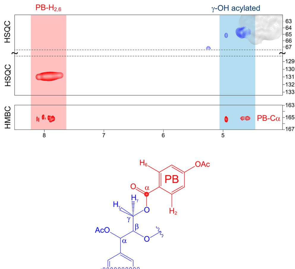
Figure 3. Section of the HMBC spectrum ( \delta_C/\delta_H 163–167/4.0–8.5) of acetylated coconut coir MWL (in CDCl_3 ) showing the main correlations for the carbonyl carbon of the p -hydroxybenzoates acylating the \gamma -positions of the lignin side chains. Appropriate sections of the HSQC spectrum showing the C_\gamma – H_\gamma correlations of the acylated lignin \gamma -carbon ( \delta_C 62–68) and the C_{2,6} – H_{2,6} correlations of p -hydroxybenzoates ( \delta_C 128–133) are also depicted.
