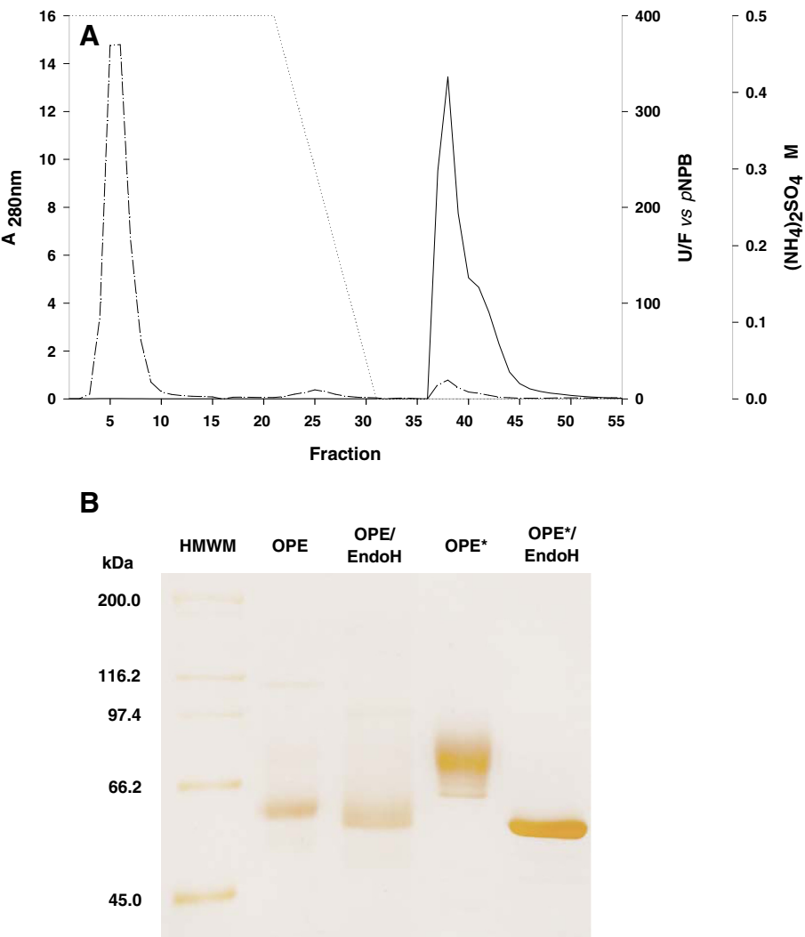
Figure 2 Enzyme purification. Hydrophobic interaction chromatography profile ( A ): units per fraction (—), A280nm (-----) and gradient (.....). SDS-PAGE for native and recombinant purified proteins before and after treatment with endoglycosidase H ( B ): High Molecular Weight Marker (HMWM), native O. piceae sterol esterase (OPE), and recombinant enzyme (OPE*). Protein bands are silver stained.
