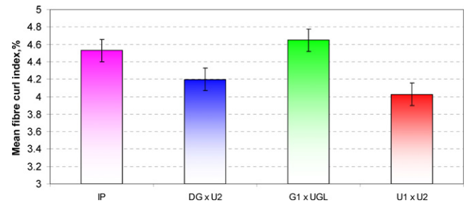
Fig. 9. Curl index of the fibers of the different eucalypt hybrid clones, allowing to give information about the fiber flexibility.
