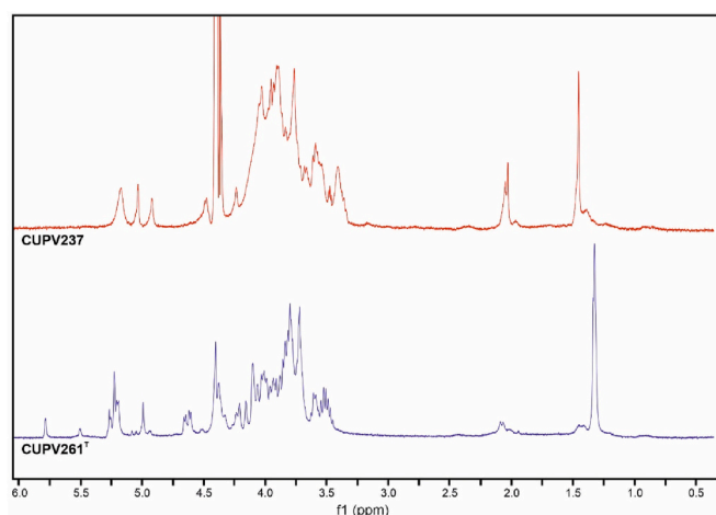
Fig. 4. 1 H NMR (500 MHz) spectra of crude EPS. The blue line corresponds to L. sicerae CUPV261 T and the red line to S. collinoides CUPV237. (For interpretation of the references to colour in this figure legend, the reader is referred to the web version of this article.)
