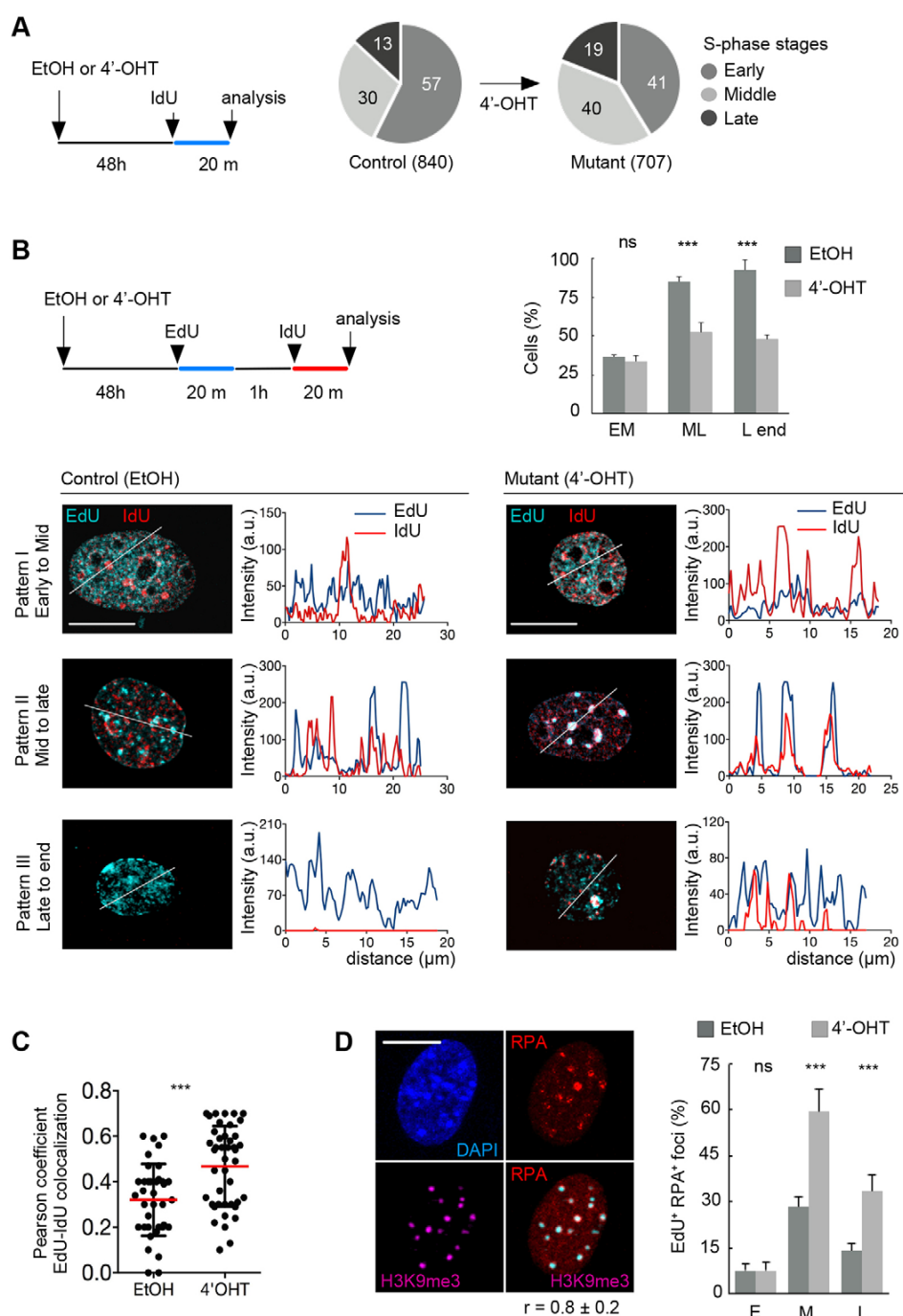
Fig. 3. Defective S-phase progression during replication of PCH. (A) Pie charts showing the proportions of cells in each stage of S-phase scored after the indicated IdU pulse. Labelled cells, in randomly selected fields, were counted (total number between brackets) until at least 50 cells were scored for the least frequent stage (late S-phase) in four independent experiments. (B) Transitions through S-phase stages. Top left, schematic of the labelling protocol. Top right, relative frequencies of the indicated transition patterns in control and mutant cultures; values show the mean±s.d. frequency from at least 50 cells per phase stage (determined at the EdU pulse) in each of three independent experiments cells. EM, ML and L end, represent early-mid, mid-late and late-to-end S-phase stages, respectively. Bottom left, representative EdU and IdU staining in control cultures showing patterns defining the indicated transition patterns. Bottom right, examples of cells with impaired transitions in mutant cultures. Bar charts are intensity profiles of immunostaining across the nucleus of representative cells at the position indicated by the line. (C) Colocalisation of EdU and IdU signals in cultures pulsed as in A. (D) Augmented frequency of mutant cells showing replicative stress at PCH. Left, representative immunofluorescence images of a mid-S-phase mutant cell showing (partial) colocalisation of RPA and the PCH marker H3K9me3; the Pearson coefficient, r , for RPA–H3K9me3 signal colocalisation (at least 50 double-positive cells in each of two experiments) is shown. Right, distribution of RPA-immunoreactive cells in each of S-phase stages. E, M and L represent early, mid and late S-phase stages, respectively. Data are mean±s.d.; n=3 (C,D). *** P\leq 0.006 ; ns, not significant ( P\geq 0.05 ). Scale bars: 10 μm.
