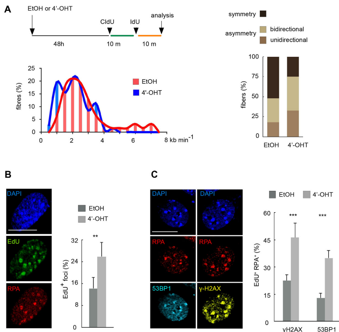
Fig. 2. Defective DNA replication and DNA damage in unperturbed RING1A- and RING1B-depleted cells. (A) Top left, schematic of the pulse experiment with thymidine analogues for DNA fibre analysis; bottom, distribution of progression speed in single DNA fibres in mutant (treated with 4'-OHT) and control (treated with EtOH) cultures. At least 150 fibres were counted for each condition in three independent experiments. The bar charts (right) show the proportions of fibres replicating symmetrically (with equal length bidirectional tracks) or asymmetrically, with uni- and bi-directional tracks. At least 80 fibres were scored for each condition in two independent experiments. (B) Replicative stress assessed by immunodetection of chromatin-bound RPA32 (left) showing an increased frequency of double EdU + , RPA + cells in mutant cultures. (C) Increased DSBs in replicative cells indicated by cells showing \gamma H2AX, 53BP1 and RPA labelling (left); bar charts display the frequencies of triply labelled cells among, at least, 100 EdU + and RPA + doubly stained cells. Bar charts are mean \pm s.d. The number of independent experiments was n=4 (B), n=3 (C). ** P=0.01 ; *** P\leq 0.003 ; ns, not significant ( P\geq 0.05 ). Scale bars: 10 \mu m.
