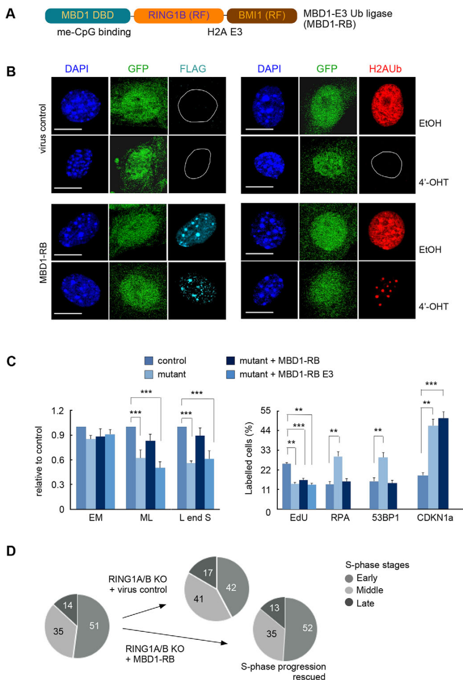
Fig. 5. Targeting RING1B-dependent H2AK119Ub monoubiquitylation to PCH rescues S-phase progression. (A) Cartoon depicting the fusion protein used to target a histone H2A
