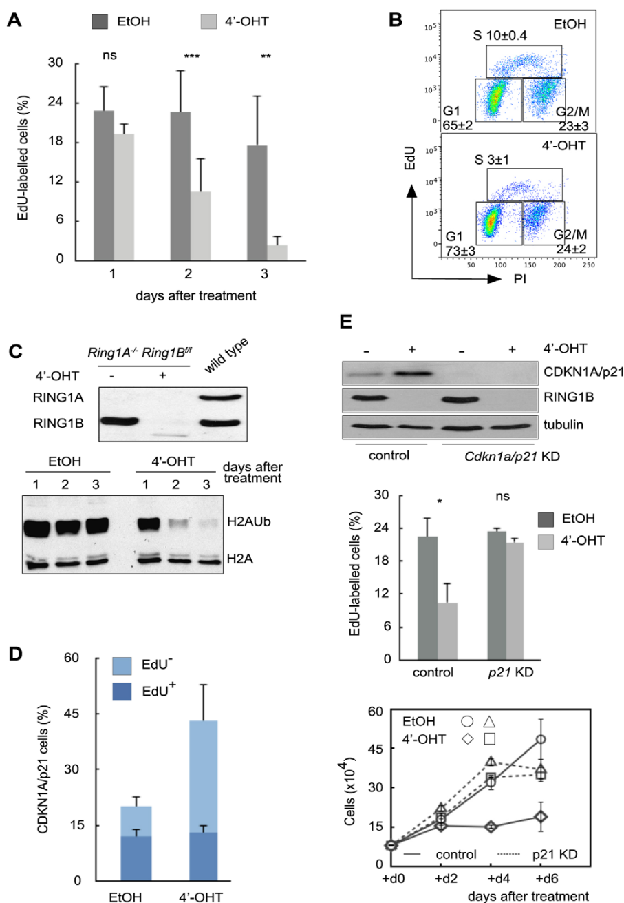
Fig. 1. Acute proliferative arrest of RING1A- and RING1B-deficient cells.
