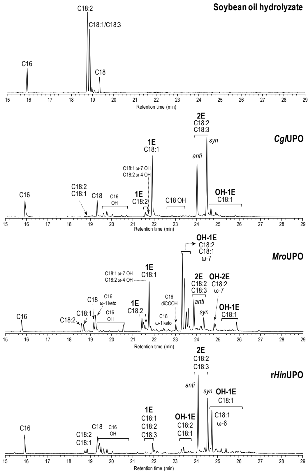
Supplementary Figure S8. GC-MS analysis of reactions of soybean oil hydrolyzate with Cg/UPO , MroUPO and rHinUPO (100 nM), showing monoepoxides and diepoxides (including syn and anti isomers from linoleic acid; 1E and 2E, respectively) and other oxygenated (hydroxy, OH; keto; and carboxy, COOH) derivatives. Control chromatogram is also shown in the top.
