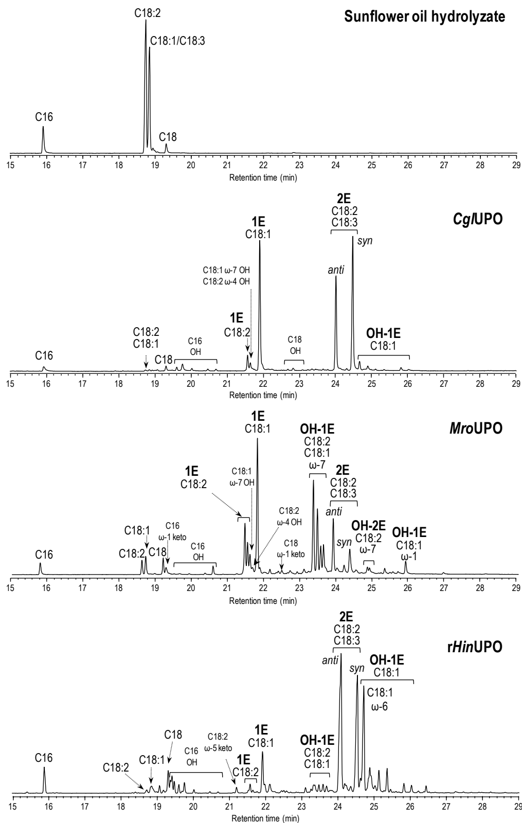
Supplementary Figure S7. GC-MS analysis of reactions of sunflower oil hydrolyzate with Cgl UPO, Mro UPO and rHin UPO (100 nM), showing monoepoxides and diepoxides (including syn and anti isomers from linoleic acid; 1E and 2E, respectively) and other oxygenated (hydroxy, OH; and keto) derivatives. Control chromatogram is also shown in the top.
