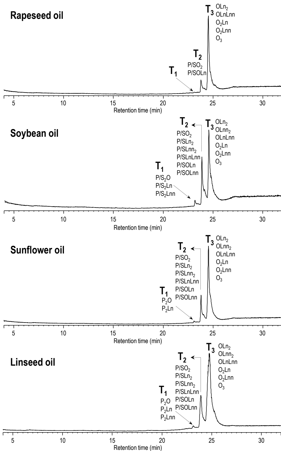
Supplementary Figure S1. GC-MS analysis of “intact” oils showing the fatty acid composition of triglycerides containing one ( T 1 ), two ( T 2 ) and three ( T 3 ) unsaturated fatty acids, in rapeseed, soybean, sunflower and linseed oils. Fatty acid abbreviations: P, palmitic acid; S, stearic acid; O, oleic acid; Ln, linoleic acid; and Lnn, α-linolenic acid.
