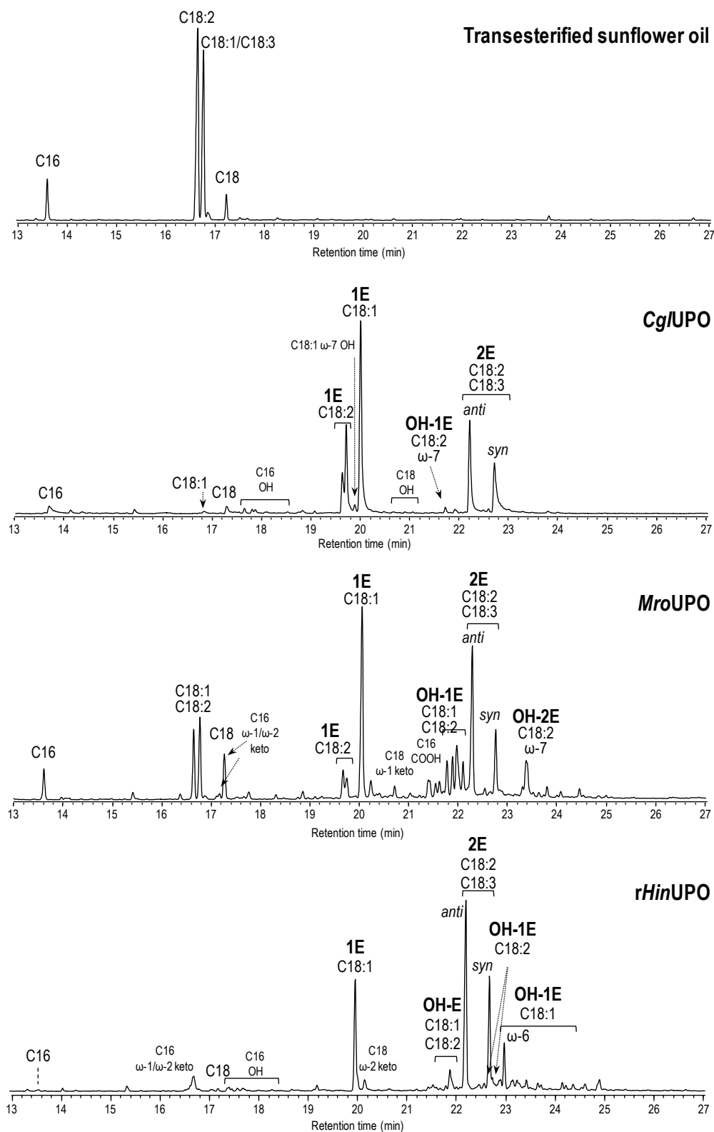
Supplementary Figure S11. GC-MS analysis of reactions of transesterified sunflower oil with CglUPO , MroUPO and rHinUPO (0.5 μM), showing monoepoxides and diepoxides (including syn and anti isomers from linoleic acid; 1E and 2E, respectively) and other oxygenated (hydroxy, OH; keto; and carboxy, COOH) derivatives of methyl esters. Control chromatogram is also shown in the top.
