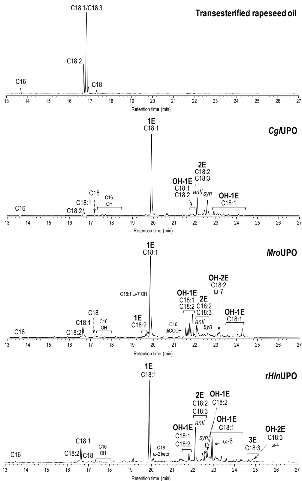
Supplementary Figure S10. GC-MS analysis of transesterified rapeseed oil (0.1 mM total fatty-acid concentration) reactions with Cgl UPO, Mro UPO and rHin UPO (0.5 \mu M), showing monoepoxides, diepoxides (including syn and anti isomers from linoleic acid) and triepoxides (1E, 2E and 3E, respectively) and other oxygenated (hydroxy, OH; and keto) derivatives (often combined in the same compound). Control chromatogram is also shown in the top.
